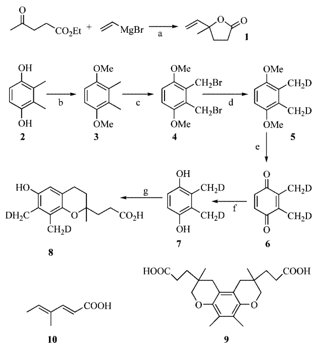
Scheme 1. a) THF, 2 h, 57%; b) NaH, DMF then MeI, 4 h, 93%; c) NBS, (Bz 2 ) 2 O 2 , CCl 4 , reflux, 3 h, 78%; d) LiAlD 4 , THF, reflux, 3 h, 88%; e) CAN, CH 3 CN/H 2 O, 20 min, 88%; f) NaBH 4 , MeOH/H 2 O, 0 °C, 20 min, 93%; g) 1 , ZnCl 2 , cat. HCl conc , 1,4-dioxane, reflux 2 h, 42%.
