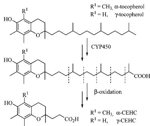
Figure 1. \alpha - and \gamma -CEHC formation from \alpha - and \gamma -tocopherol by cytochrome P450 Cyp4F2 enzyme followed by \beta -oxidation. [4]
